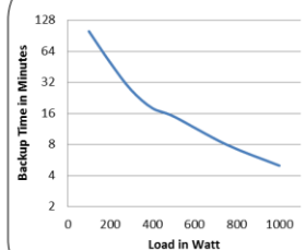
Runtime curve
