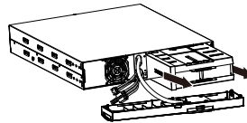
Battery Set with 3x 12V/7Ah batteries (Plug-and-Play solution incl. case and cabling to change internal bat. Set of VFI 1000RT LCD) Datasheet: Link Item No.: to be checked
